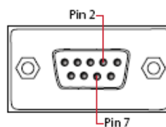
9-pin female connector, front-side view
